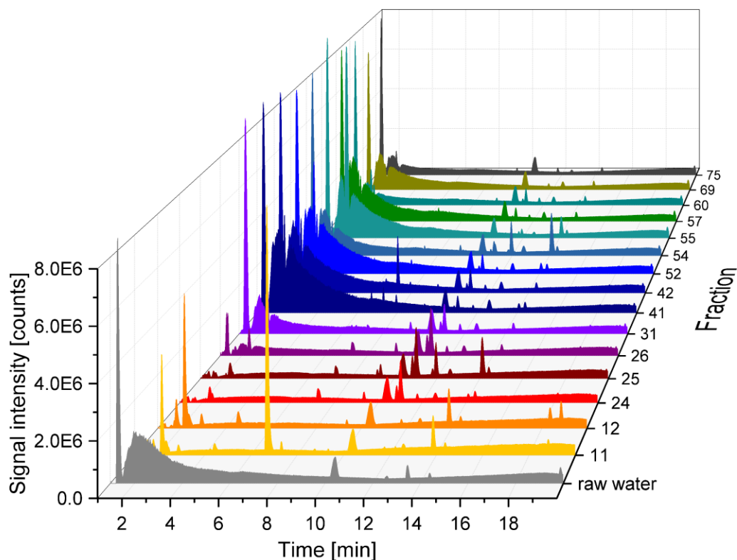
Figure 63: Base peak chromatogram of FFIZE separated samples, BPCs in the range of 80 - 1200 \pm 0.01 m/z analyzed by HPLC-QTOF-MS in the positive ionization mode. A pH gradient of pH 5 at fraction 19 - 30 to pH 9 at fraction 83 - 94 was applied and the sample injected at fraction 71 - 85. Further parameters, see Section 6.3.1.
