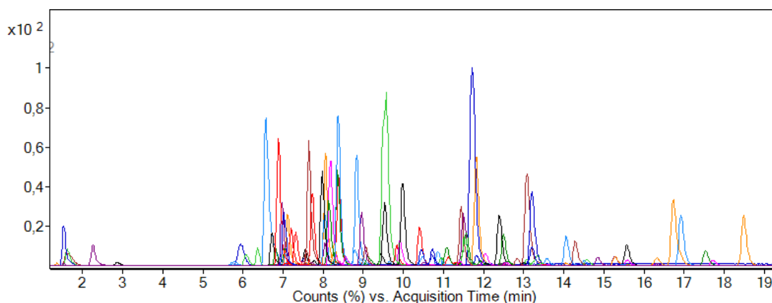
Figure 54: Extracted ion chromatograms of 92 compounds in the reference mixture at a concentration of 5 µg/L analyzed by HPLC-QTOF-MS in the positive ionization mode within 20 min. Further parameters see text.
