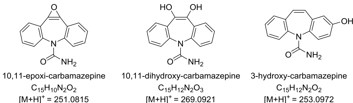
Figure 5: Metabolites known from literature 93-94 , were analyzed but not detected in samples.
