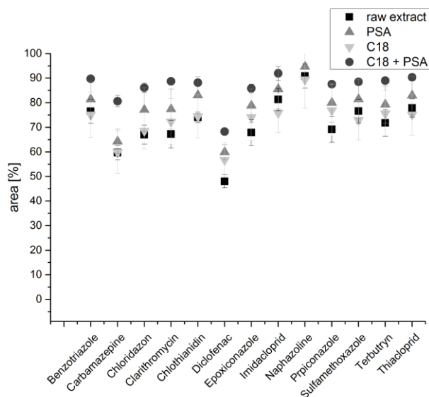
Figure 2: Signal intensities of analytes spiked to midge larvae extracts after extraction and before analysis. Signal intensities in % are calculated compared to analyte signals in MeOH at the same concentration.
