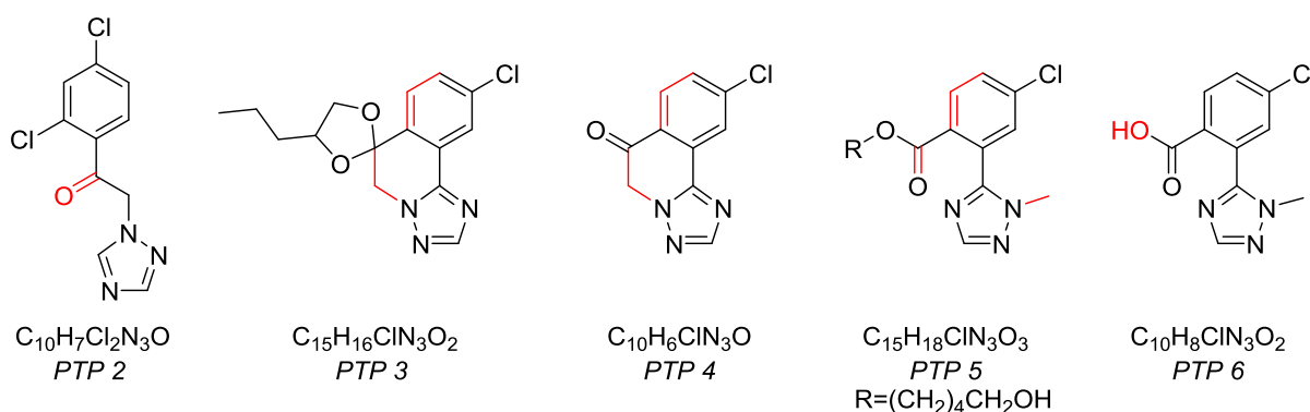
Figure 35: Molecular structure of propiconazole and photo transformation products PTP , changes highlighted in red. PTP 2 1-(2,4-dichlorophenyl)-2-(1H-1,2,4-triazol-1-yl)ethane-1-one, PTP 3 9-chloro-4'-propyl-5H-spiro[[1,2,4]triazolo[5,1-a]isoquinoline-6,2'-[1,3]dioxolane], PTP 4 9-chloro-[1,2,4]triazole[5,1-a]isoquinoline-6(5H)-one, PTP 5 4-hydroxybutyl 4-chloro-2-(1-methyl-1H-1,2,4-triazol-5-yl)benzoate and PTP 6 4-chloro-2-(1-methyl-1H-1,2,4-triazole-5-yl)benzoic acid.
