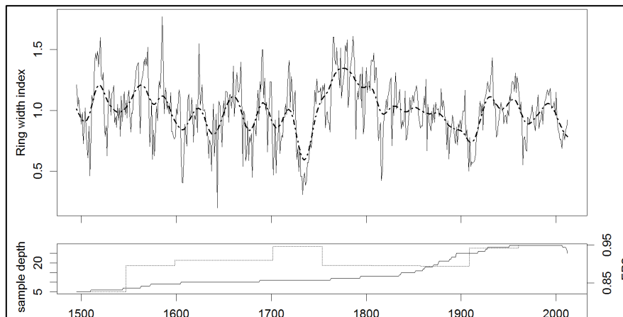
Figure 1: Tree ring width chronology from Picea balfouriana (SE Tibetan Plateau) with 32 years running spline. Solid line in the lower panel represents the sample depth, dotted curve the EPS.
