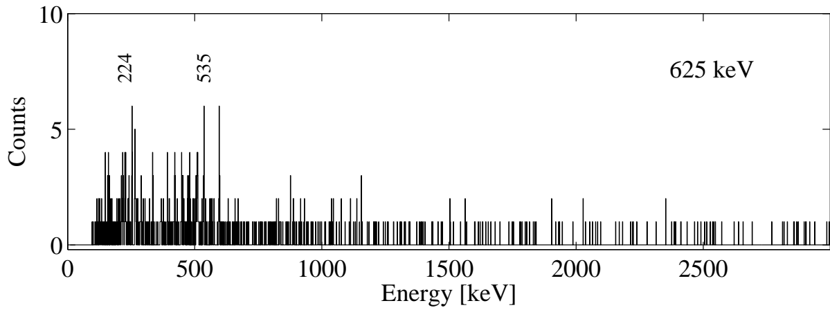
Figure 6.14: Example for coincidence spectra of low intensity.
