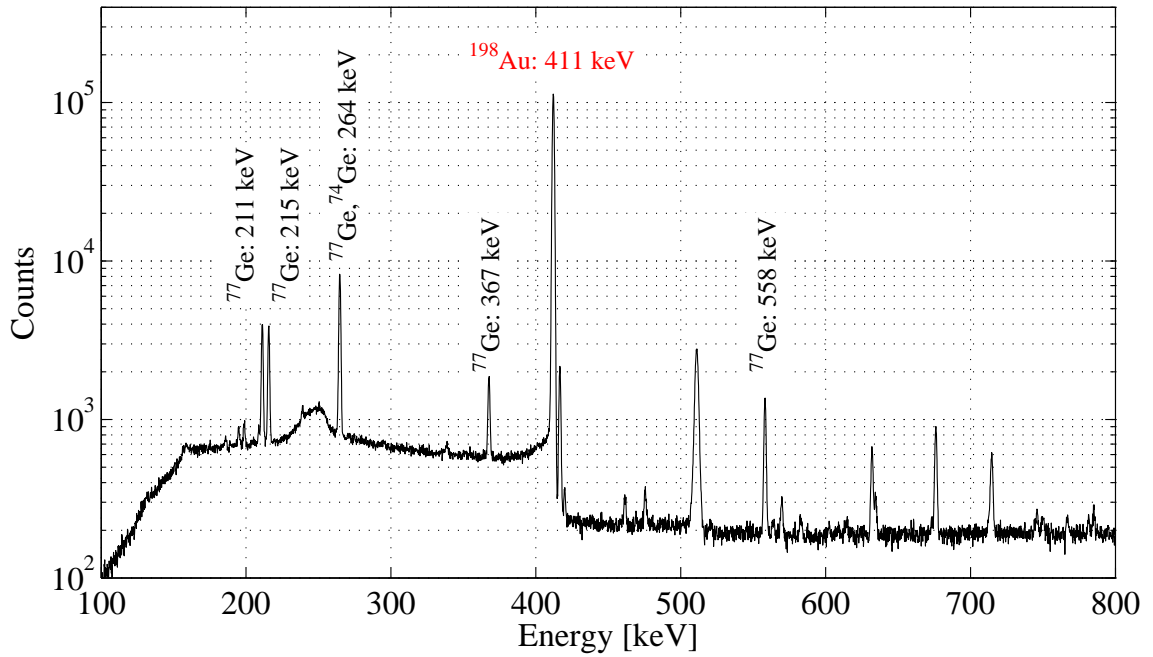
Figure 3.2: Spectrum with ^{77}\text{Ge} and ^{198}\text{Au} decay lines used to evaluate the cross section.
