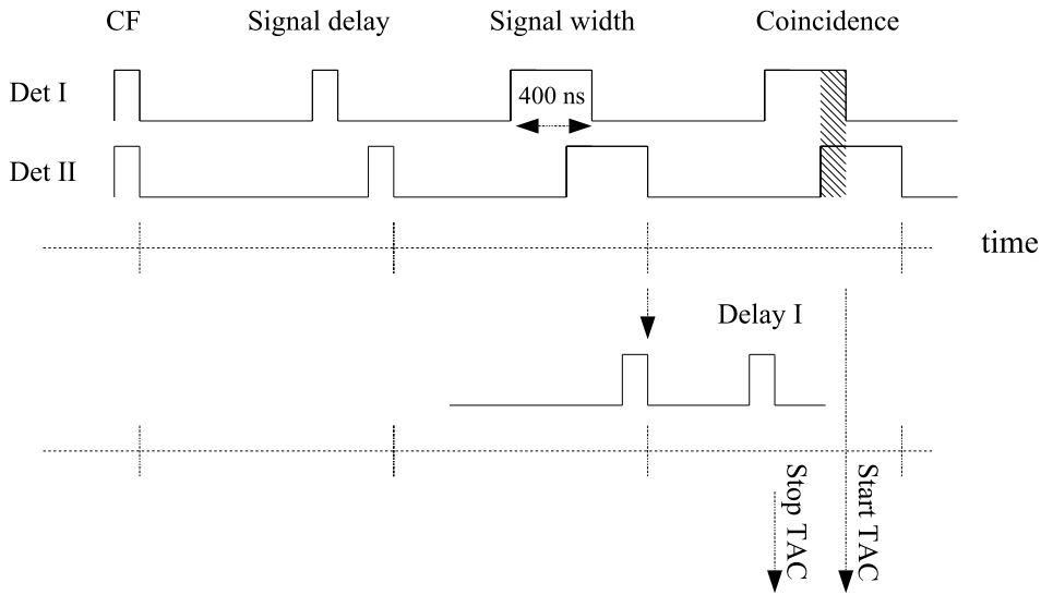
Figure 6.4: Logic pulses for the coincidence trigger and TAC start/stop.
