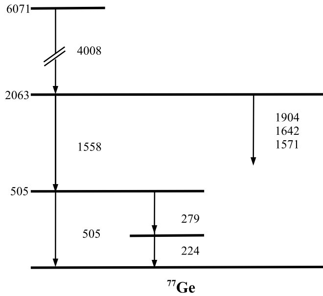
Figure 6.16: Decay branches following the 4008 keV transition.
