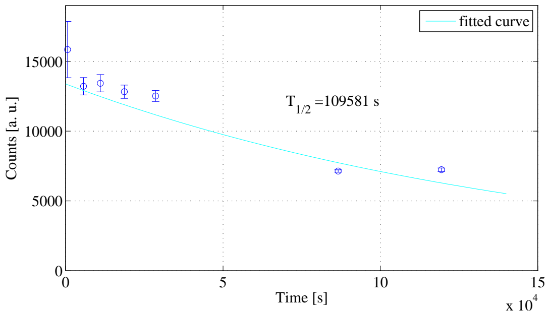
Figure 4.2: Decay curve of the 520 keV peak. The fit is not consistent with the half-life of ^{77}\text{Ge} . The peak contains a strong contribution by the longer lived ^{77}\text{As} isotope ( T_{1/2} = 38.8 h).
