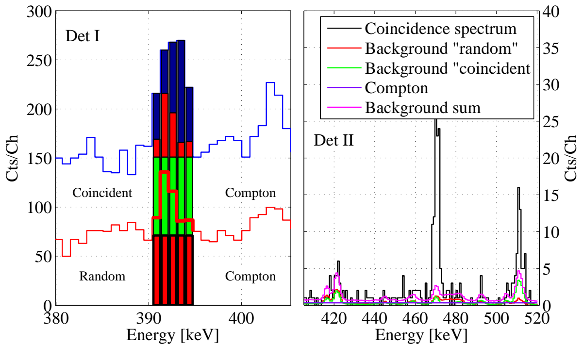
Figure 6.12: Quantitative determination of the background in coincidence spectra. The left side presents the region selected for analysis in detector I with the different background contributions. The right side shows the corresponding background in detector II.
