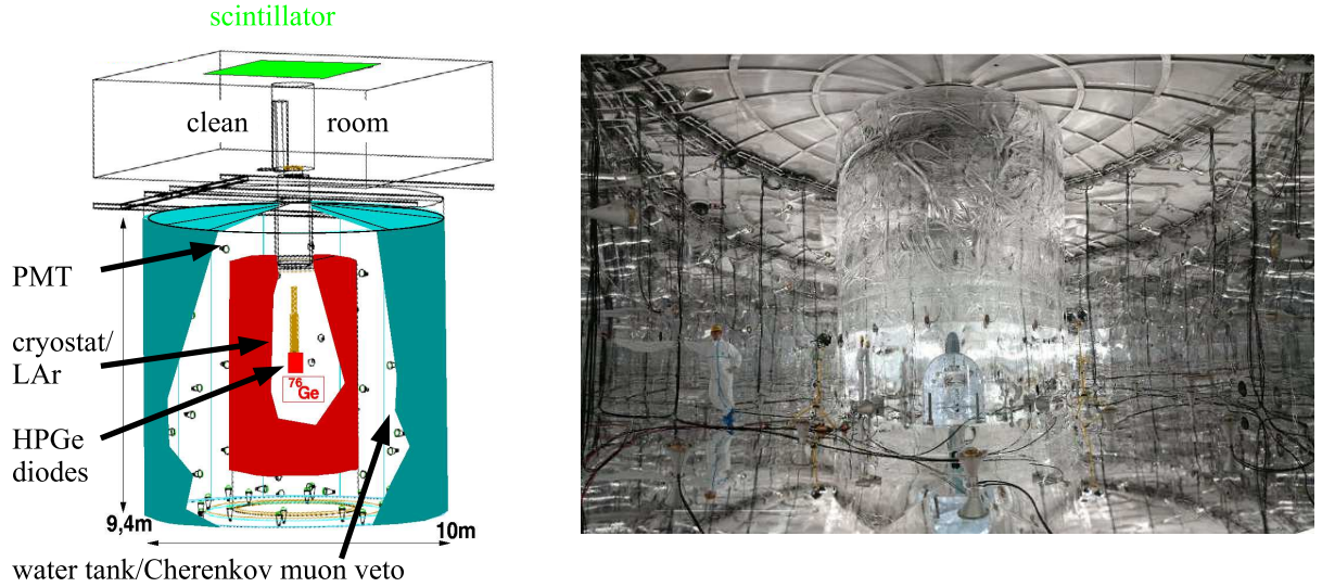
Figure 1.2: Left: Setup of GERDA. Right: Water tank, the walls and the floor are covered with reflective foil for the active muon veto.
