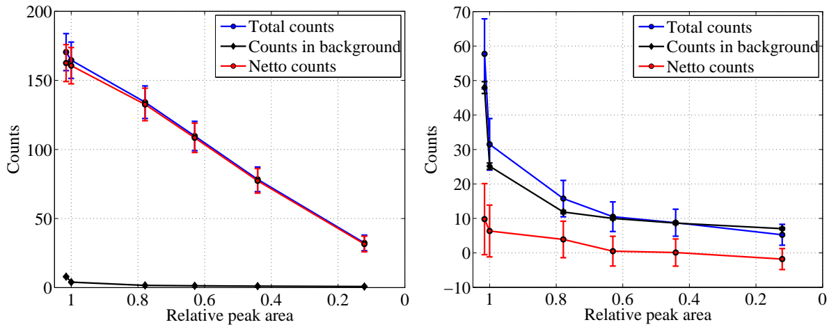
Figure 6.17: Determination of coincidences by count ratios. The number of counts plotted against the relative peak area (defined as ratio of true coincidences with cut “ABx”/“AB2”, table B.1) gives a straight line if two peaks are in coincidence. Left: Peak at 862 keV in detector II coincident with peak at 5050 keV in detector I. Right: Hydrogen peak at 2223 keV in detector II coincident with peak at 862 keV in detector I. Since this transition has no coincidences at all, the shape of the blue curve is typical for events of pure random coincidence.
