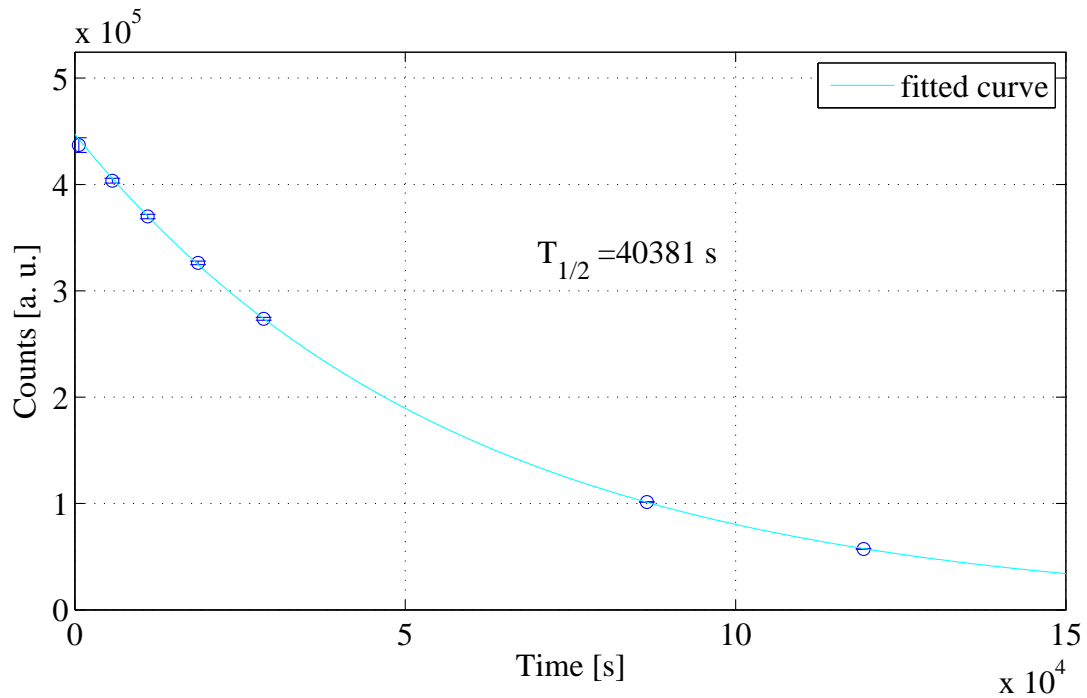
Figure 4.1: Decay curve of the 558 keV peak. The fitted exponential function is consistent with the half-life of ^{77}\text{Ge} .
