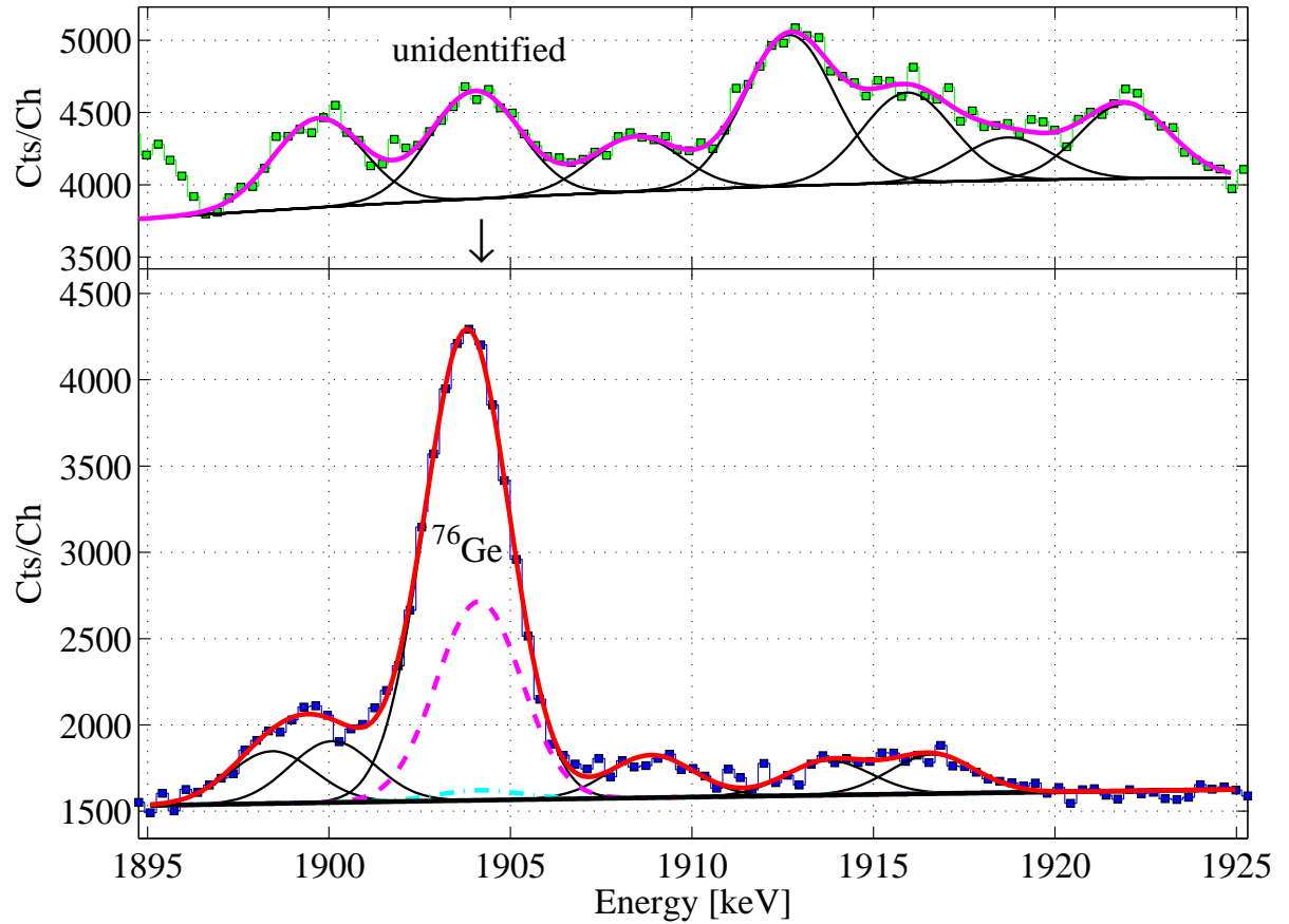
Figure 6.2: Subtraction of an unidentified peak. If the peak in the depleted (upper) spectrum is due to ^{74}\text{Ge}(n,\gamma) the contribution in the enriched (lower) spectrum is shown by the pink, for ^{73}\text{Ge}(n,\gamma) by the turquoise gaussian.
