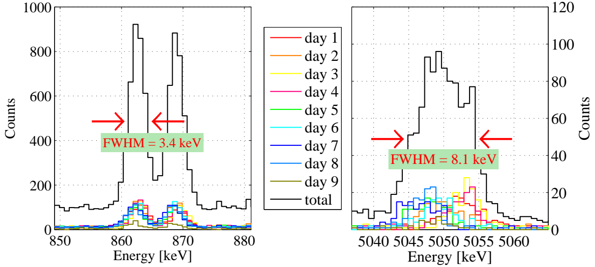
Figure 6.8: Energy drift of detector II for the peaks at 861 keV and 5049 keV. Each spectrum represents a time interval of 86 400 s. Cuts: “AB1c”.
