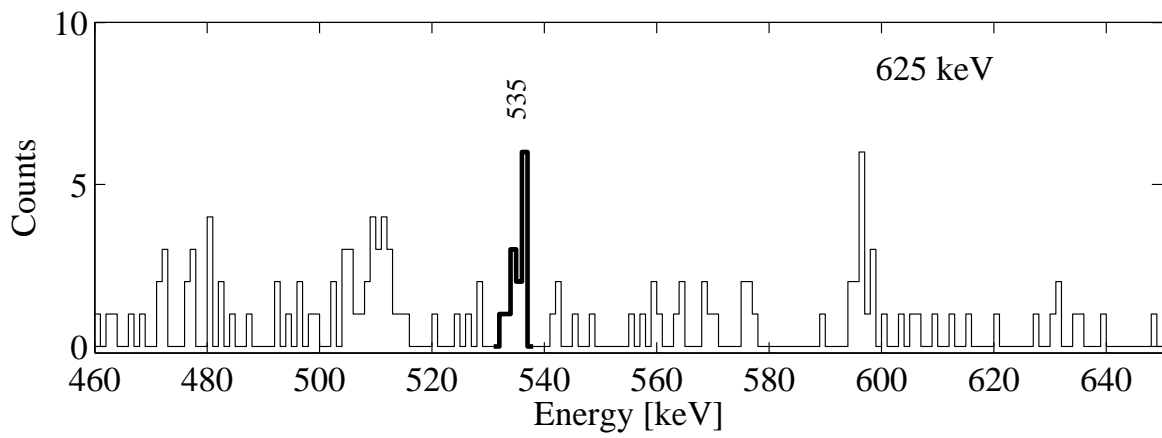
Figure 6.14: Example for coincidence spectra of low intensity.
