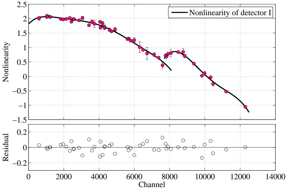
Figure 2.6: Nonlinearity of detector I in channels fitted with a polynomial of 6 th degree (lower energy region) and 4 th degree (upper energy region). The lower diagram shows the deviation of the data from the fit. Multiply with 0.5365 to obtain the nonlinearity in keV for the prompt \gamma -ray measurement in chapter 6.
