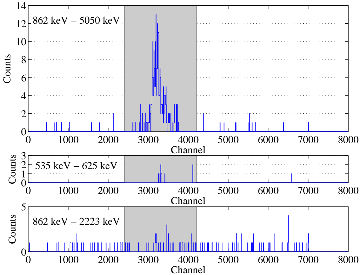
Figure 6.13: Time spectrum for three coincidence pairs. The transitions in the upper two plots are in coincidence, almost all events are within the window for true coincidences. In the lower plot the events are more equally distributed, hence it is dominated by random coincidences.
