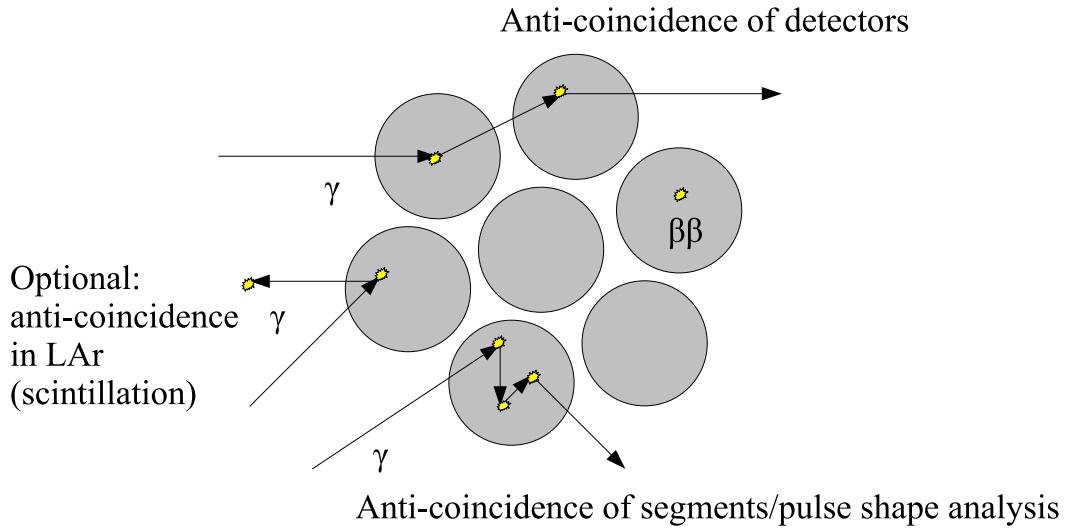
Figure 1.4: Hypothetical detector array for GERDA. While double beta decay has a single-site signature, high energetic \gamma -rays cause mostly multi-site events that can be rejected by pulse shape analysis.
