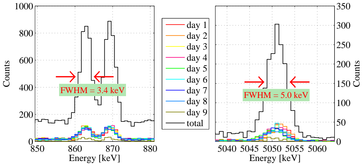
Figure 6.9: Energy drift of detector I for the peaks at 861 keV and 5049 keV. Each spectrum represents a time interval of 86 400 s. Cuts: “AB1c”.
