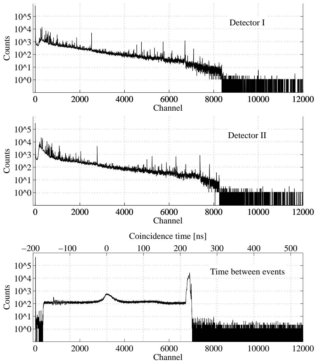
Figure 6.6: The upper two plots show the spectra recorded with detector I and II. The lower spectrum shows the time differences between events in the two detectors. The peak at “coincidence time” = 0 ns is due to real coincidences, the flat component arises from random coincidences.
