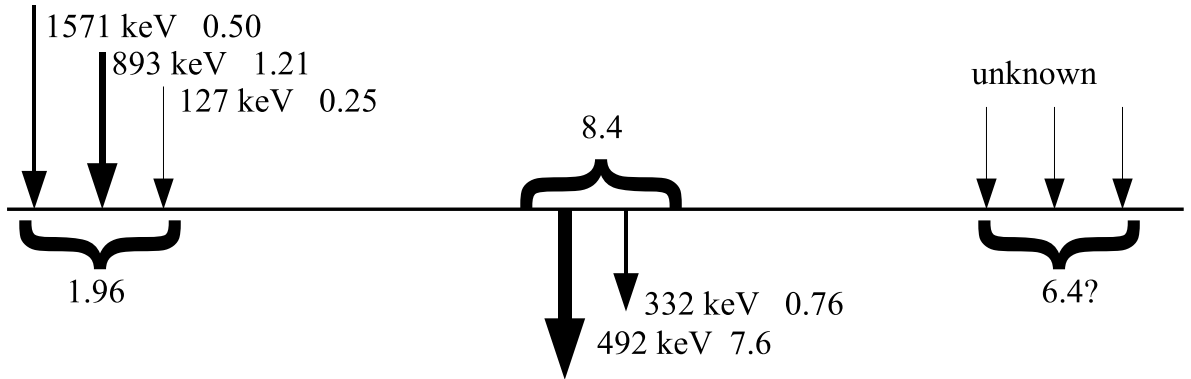
Figure 6.18: Origin of the difference between measured and simulated intensities. The numbers represent the relative intensities.
