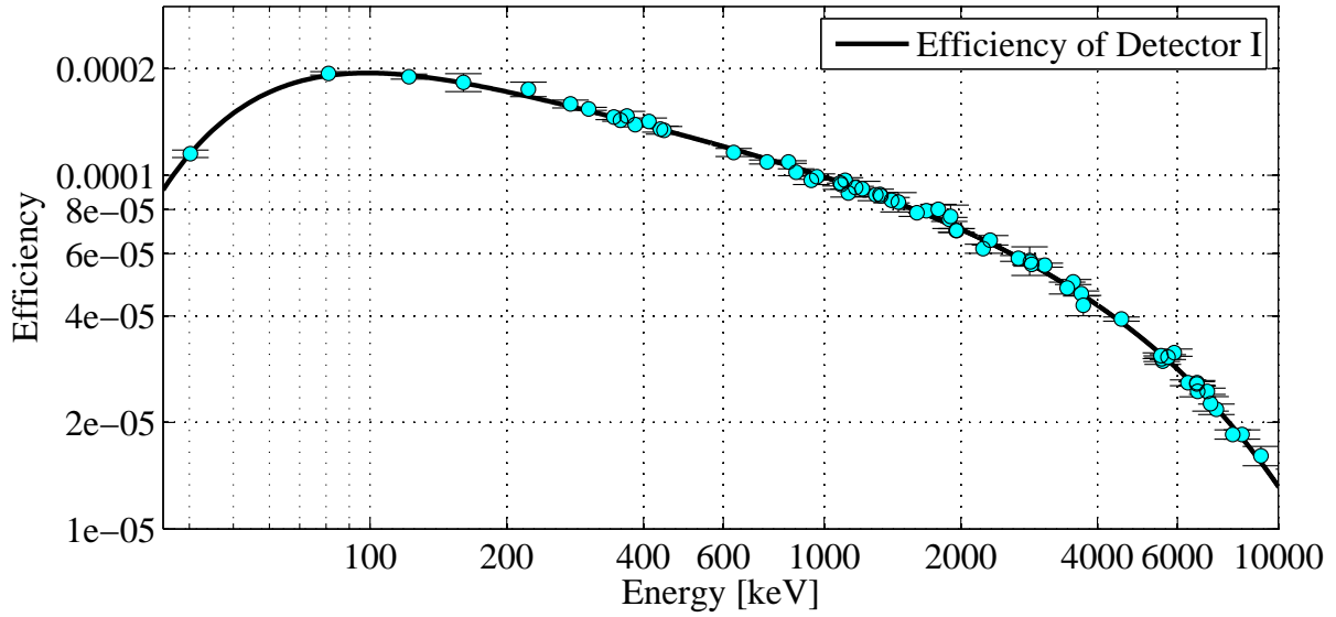
Figure 2.8: Efficiency of Detector I [10].
