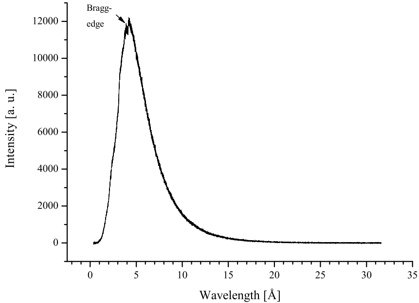
Figure 2.5: Measured wave length spectrum at the target position. At \lambda = 4,05 \text{ \AA} the Bragg edge used for calibration is visible.
