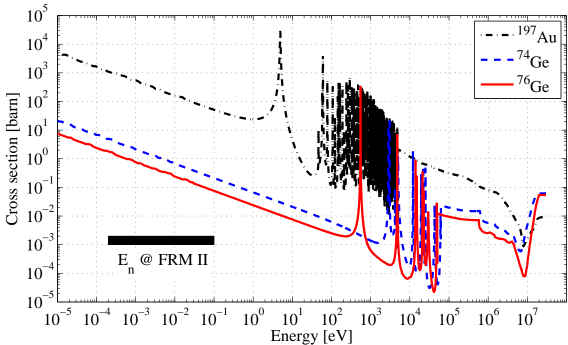
Figure 3.3: Neutron capture cross sections of ^{74}\text{Ge} , ^{76}\text{Ge} and ^{197}\text{Au} [3]. The black bar represents the energy range of the neutron beam available at the PGAA instrument.
