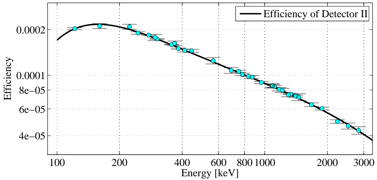
Figure 2.9: Efficiency of Detector II [10].
