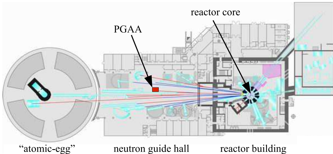
Figure 2.3: Neutron guide hall at the FRMII [2]. The PGAA instrument is located at the end of neutron guide NL4b.
