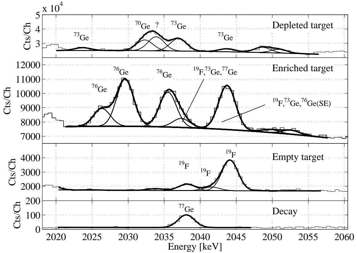
Figure 6.20: Spectra of the depleted, enriched (prompt and decay) and empty target in the region of interest around 2039 keV. The spectra were normalized for comparison in the way that the most important isotope occurs with the same intensity as in the enriched spectrum (depleted: ^{74}\text{Ge}(n,\gamma) , empty: ^{19}\text{F}(n,\gamma) , decay: ^{77}\text{Ge} decay).
