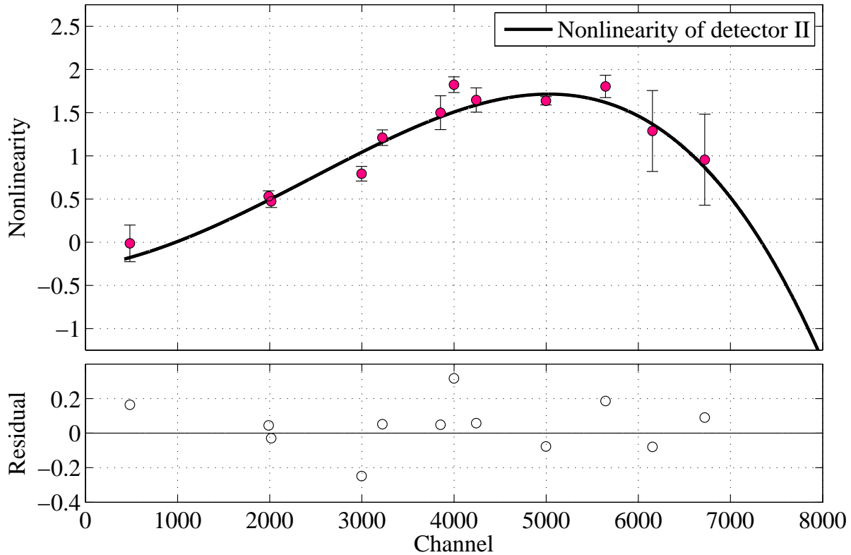
Figure 2.7: Nonlinearity of detector II in channels fitted with a polynomial of 4 th degree. The lower diagram shows the deviation of the data from the fit. Multiply with 0.325 to obtain the nonlinearity in keV for the prompt \gamma -ray measurement in chapter 6.
