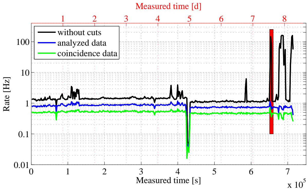
Figure 6.5: Rate of coincident events during the measurement. The raw data (black) show peaks caused by electronic noise that can be suppressed applying different cuts (blue, green). The corresponding cuts can be found in table 6.5. The remaining dips are due to neutron beam shut downs for testing and refilling of nitrogen in the dewars. For analysis only data left from the red bar ( t = 650\,986 s) were taken into account. The bin width is 1800 s.
