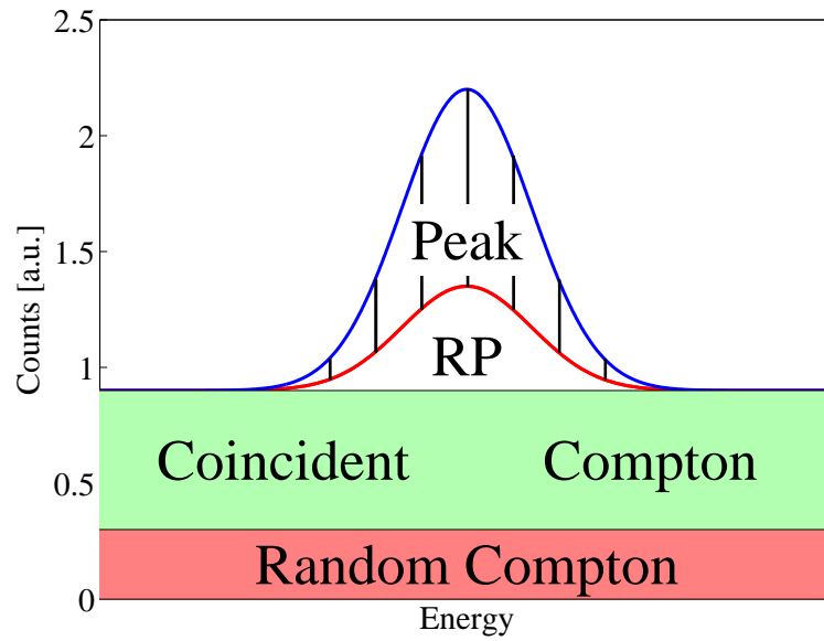
Figure 6.11: Schematic view of the background composition, RP denotes “random peak”.
