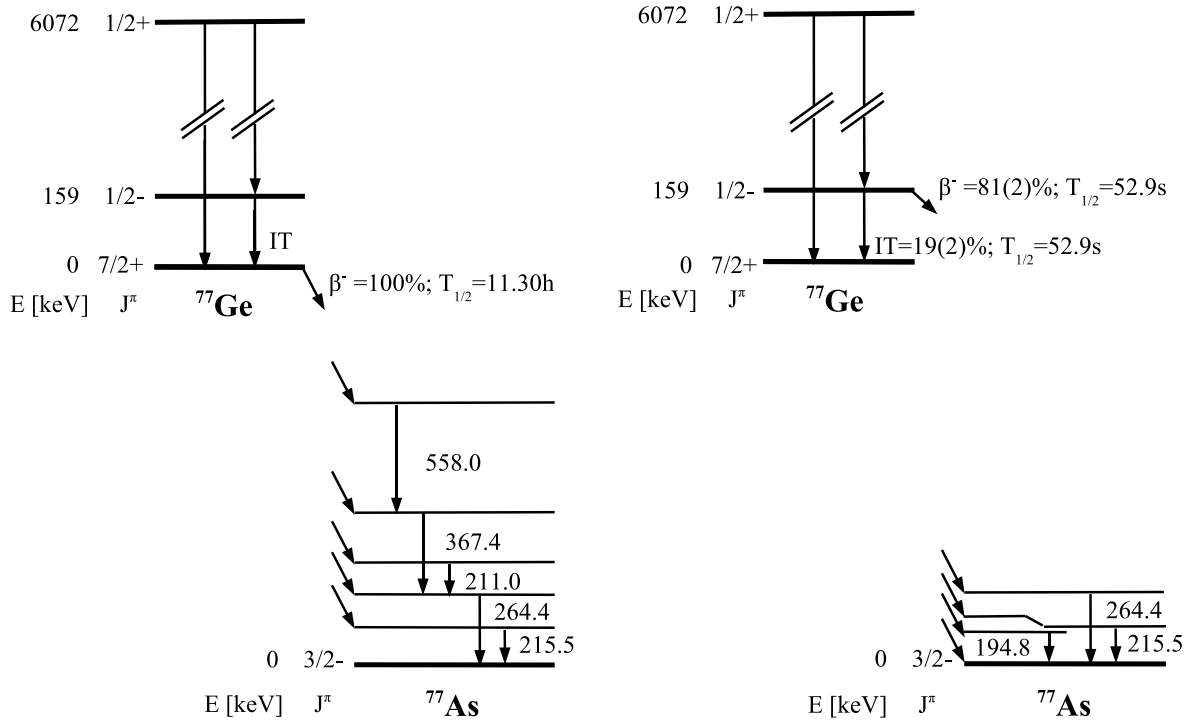
Figure 3.1: Decay scheme of the ground state (left) and the isomeric state (right).
