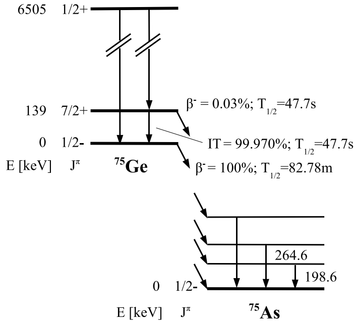
Figure 3.4: Decay scheme of ^{75}\text{Ge} .
