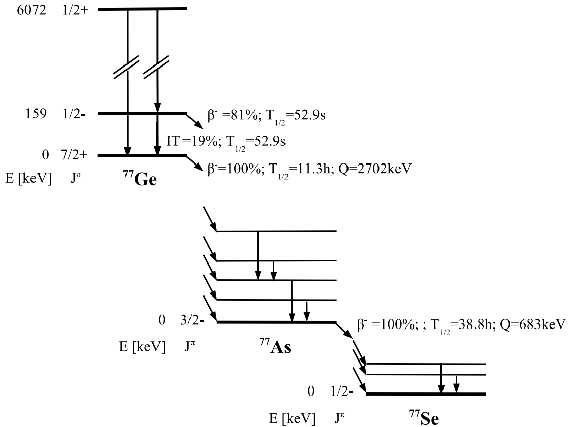
Figure 1.5: Decay chain after neutron capture on ^{76}\text{Ge} .
