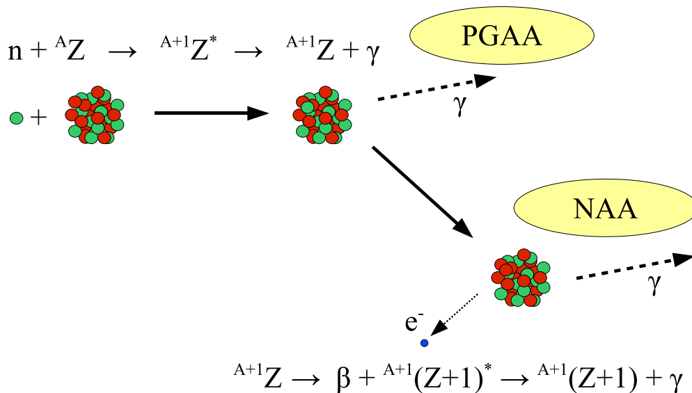
Figure 2.1: PGAA principle.
