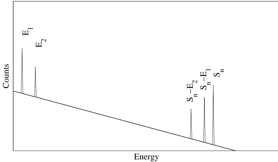
Figure 2.2: Sketch of a typical PGAA spectrum.
