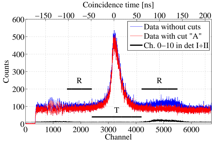
Figure 6.7: Time spectrum with cut “A” and without cuts on the energy spectra. The bump right of the coincidence peak disappears setting cut “A”. If only channels 0-10 are selected in detector I+II the bump is reproduced (plotted with offset of 10 counts/ch.). Hence it corresponds to events with no signal in both detectors.
