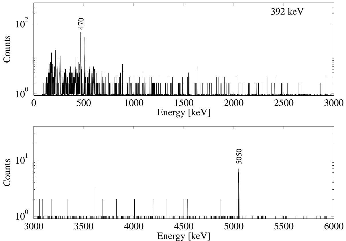
Figure 6.10: Spectrum of events coincident with the 392 keV line.
