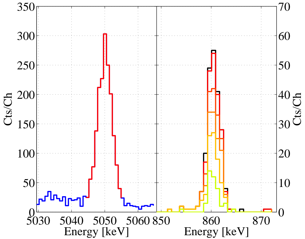
Figure B.1: Coincidence of the 5050 keV peak with the 862 keV line. The red marked area in the left spectrum (detector I) shows the channels used to plot the coincident events in detector II. The six different colors correspond to the range “AB1-6” given in table 6.4.
