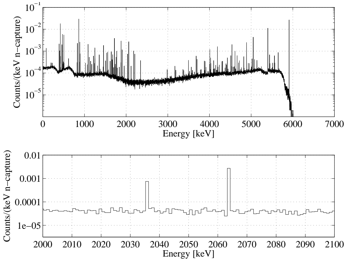
Figure 6.19: Simulated prompt spectrum in ^{77}\text{Ge} for a single phase I detector. The counts in bin 2063 represent the sum peak corresponding to the 2063.2 keV level.
