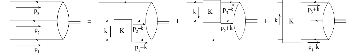
Figure 5.6.: Faddeev equation for three quark bound states. Solid lines represent the quark propagator, the box represents the diquark kernel K and the ellipse represents the Faddeev vertex function with the bound state leg depicted by a triple-line. See text for details.
