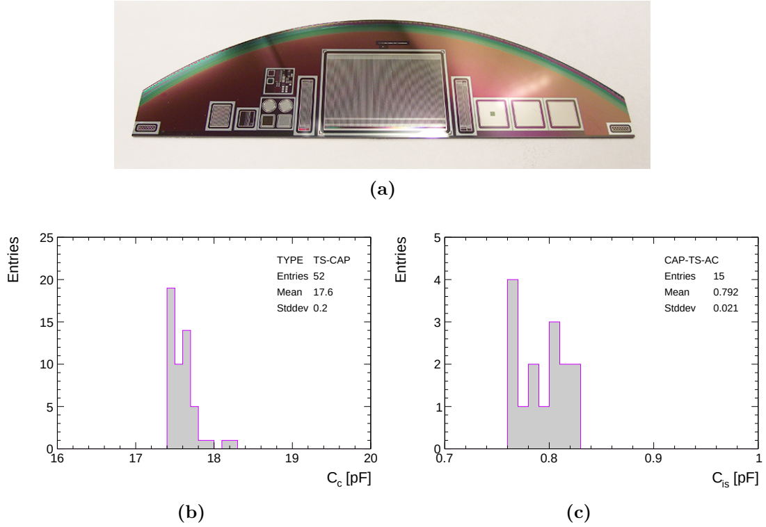
Figure 3.15.: Results of the electrical performance cross-check using CMS test-structures. (a) A photo of the CMS standard “half-moon” containing nine test structures. (b) Distribution of the measured coupling capacitance. (c) Distribution of the measured interstrip capacitance.
