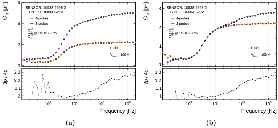
Figure 4.65.: Frequency dependence of the interstrip capacitance measured on the CBM06H6 sensor in different configurations: comparison of (a) 4-probe and 3-probe configurations, (b) 4-probe and 2-probe configurations. The capacitance measured in the 4-probe configuration is the interstrip capacitance to one neighbor, while the other configurations include contributions from the remaining strips.
