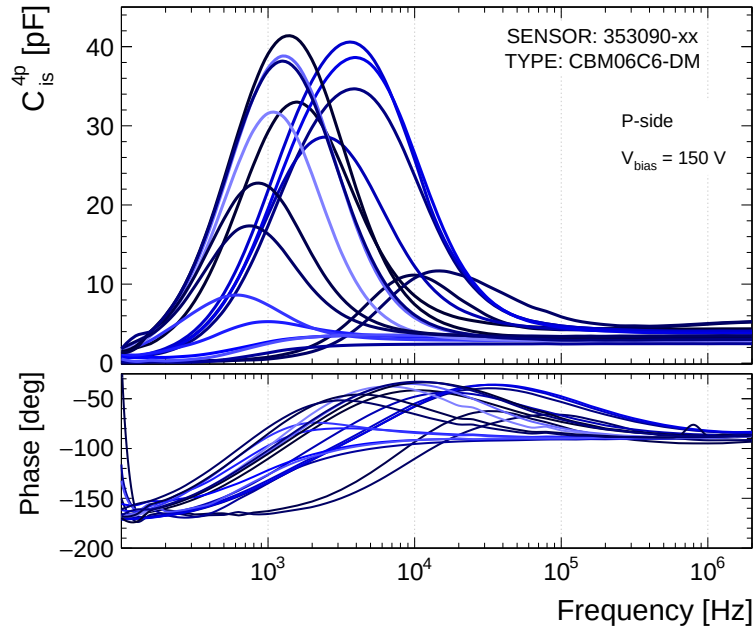
Figure 4.72.: Frequency dependence of the interstrip capacitance measured on the p side of the CBM06 sensors of batch 353090. Measurements were performed on randomly selected strips of five sensors in a 4-probe configuration. The observed shapes are explained by the low interstrip resistance, which shunts the interstrip capacitance at low frequencies.
