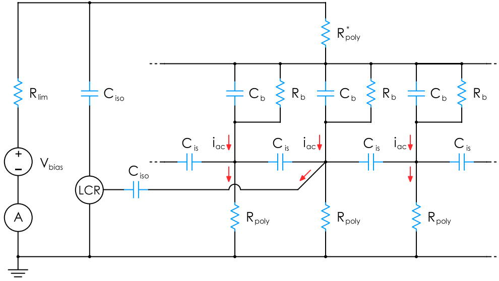
Figure 4.58.: Equivalent circuit of three strips of the CBM microstrip sensor with the LCR meter connected for the strip backplane capacitance measurement. C_b and R_b represent the backplane capacitance and the parallel resistance assigned to one strip. C_{is} is the interstrip capacitance. R_{poly}^* is the equivalent polysilicon resistor of the opposite side.
