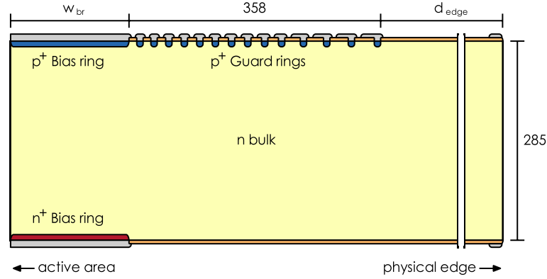
Figure 2.7.: Schematic drawing of the guard ring structure of the CBM sensor manufactured by CiS. It consists of 14 concentric rings. Distances are in \mu\text{m} . The thickness of implants and metals is increased for clarity. The active area is not shown. The distance between the metal rings is the same due to the overhang technology.
