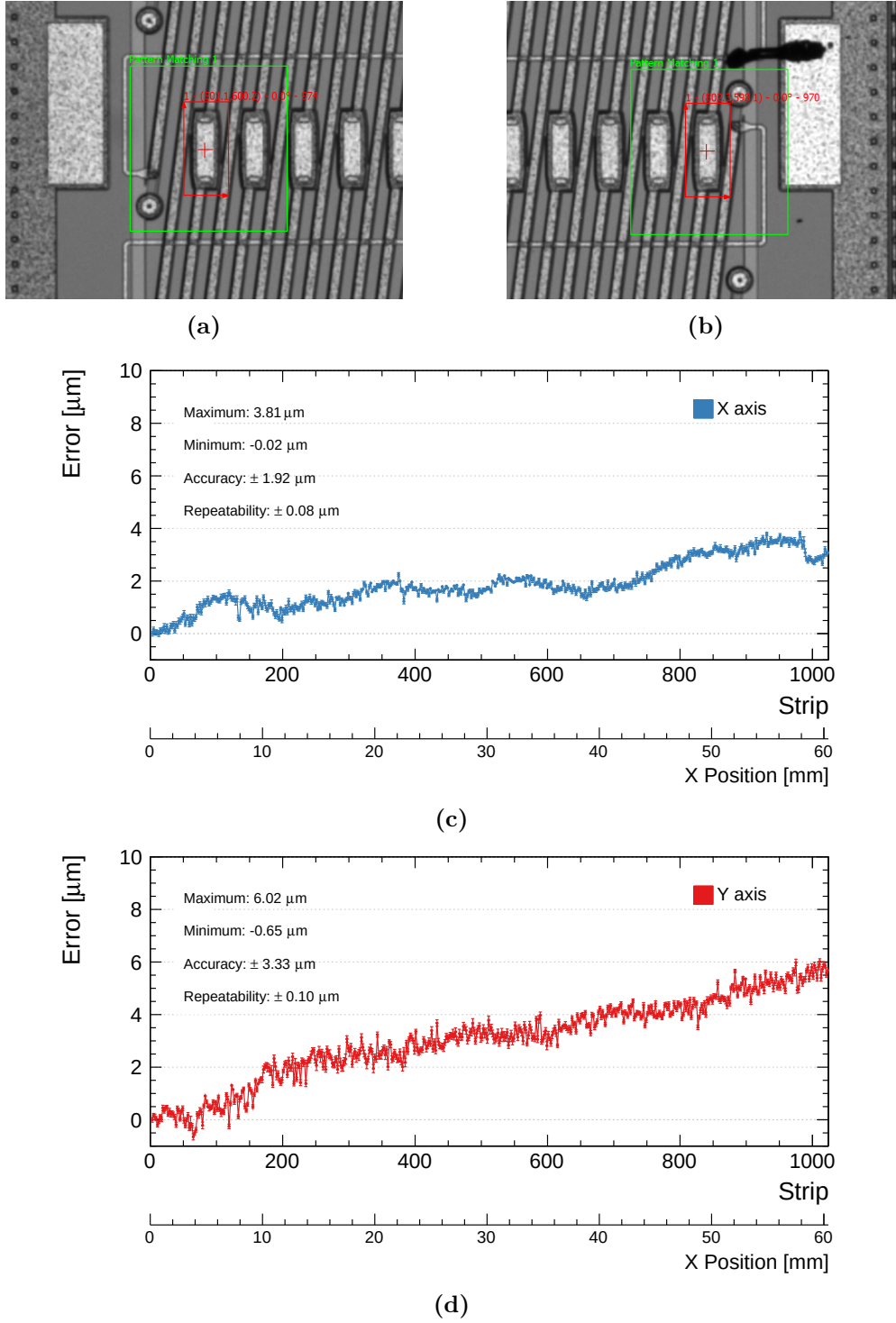
Figure 3.11.: Performance estimation of the probe station in terms of accuracy and repeatability of the positioning of the sensor under the probe needle. (a)-(b) The position of the AC pads is detected by the Pattern Matching tool. It is compared to the true position in the sensor coordinate space and positioning errors are calculated for every AC pad. (c)-(d) Positioning accuracy plots. The data points represent the average inaccuracy at the position of the AC pad, the error bars represent one standard deviation.
