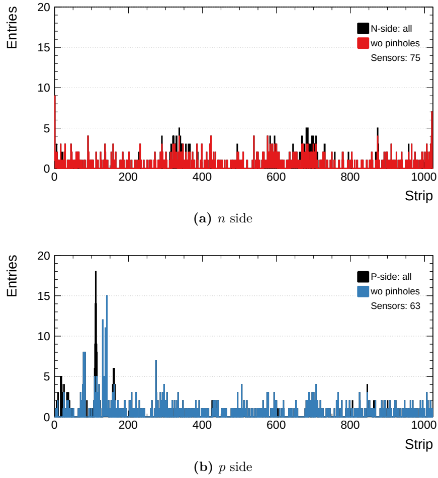
Figure 6.10.: Map of accumulated defective strips for n and p sides of the CBM sensors. The data for all sensor variants is combined. The different number of sensors for n and p sides is due to the identified contact loss for some sensors.
