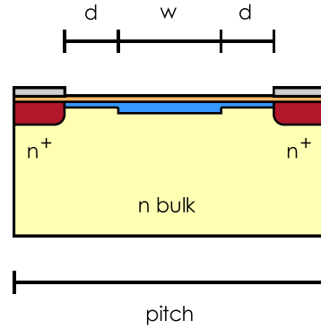
Figure 2.2.: Schematic view of the n side of the CBM microstrip sensor manufactured by CiS. The strip implant (shown in red) width is 20\text{ }\mu\text{m} ; the gap d is 9\text{ }\mu\text{m} wide and doped with boron at a peak concentration of 1 % of the main p -spray area (shown in blue) that has width w = 20\text{ }\mu\text{m} [73].
