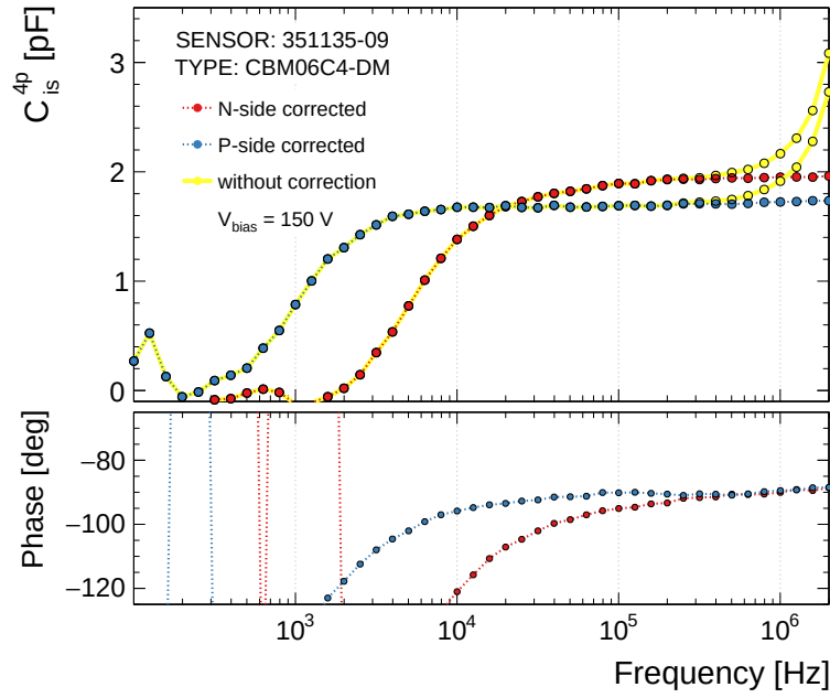
Figure 4.68.: Frequency dependence of the interstrip capacitance measured on both sides of the CBM06 sensor in a 4-probe configuration with and without correction for the gain error. On the n side the effect is more critical, while on the p side measurements can be performed at lower frequencies.
